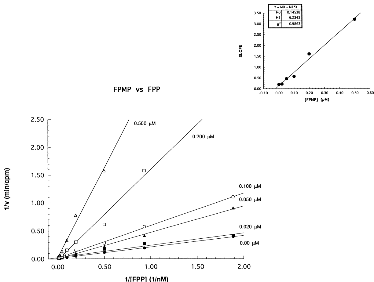
Figure 6. Lineweaver–Burk plot of competitive mFTase inhibition by FPMP (7). The values were obtained using the scintillation proximity assay as described in the experimental section, with the exception that the peptide concentration was maintained at 0.10 \mu M and the FPP concentration was varied. Enzyme rates were determined at 0, 0.02 \mu M, 0.05 \mu M, 0.10 \mu M, 0.20 \mu M, and 0.50 \mu M FPMP, as indicated on the figure.
